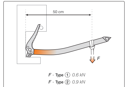
Shaft insertion strength test
