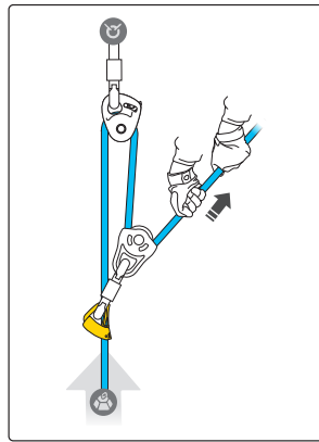
Hauling gear
