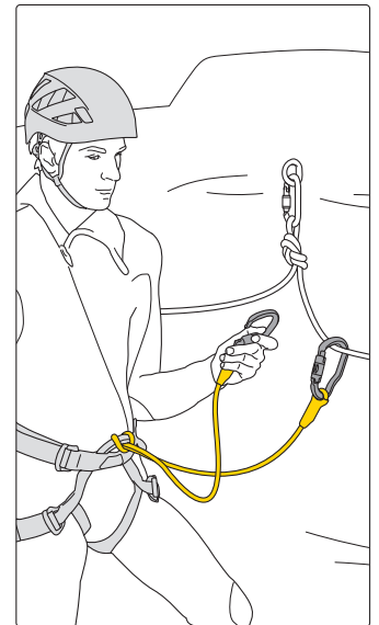
The DUAL CANYON CLUB, DUAL CANYON GUIDE and DUAL CONNECT VARIO lanyards allow positioning at the anchor and progression along a lifeline when canyoning.
