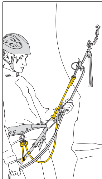
The DUAL CONNECT ADJUST and DUAL CONNECT VARIO double lanyards allows the user to tether him/herself in order to set up a rappel system when climbing or mountaineering.
