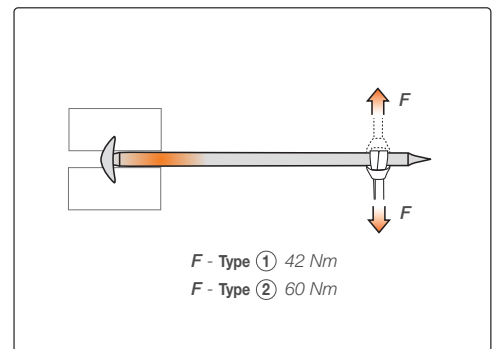
Levering test
