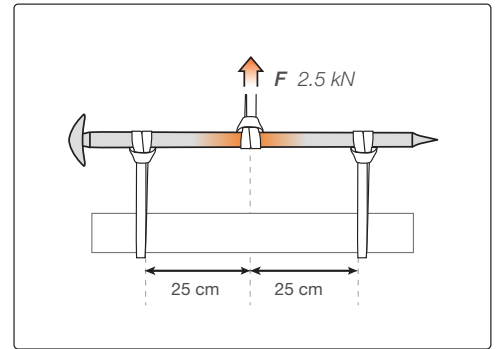
Pull test
